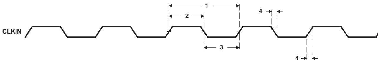
Figure 21. CLKIN Timings
